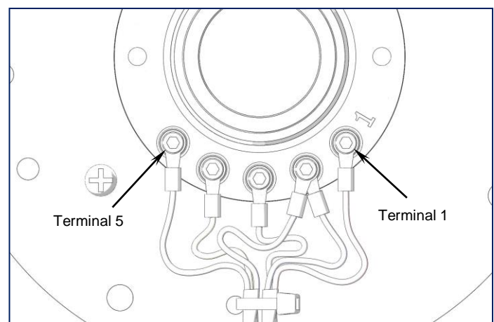
Stator Wiring Diagram
