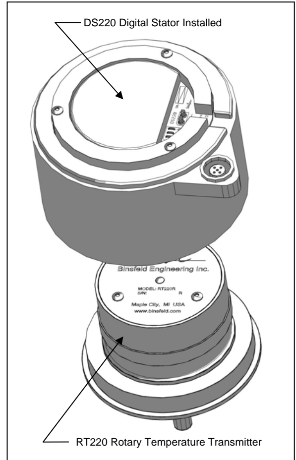
Installation Overview
