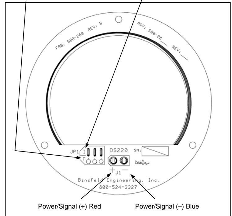
Power/Signal Connection
